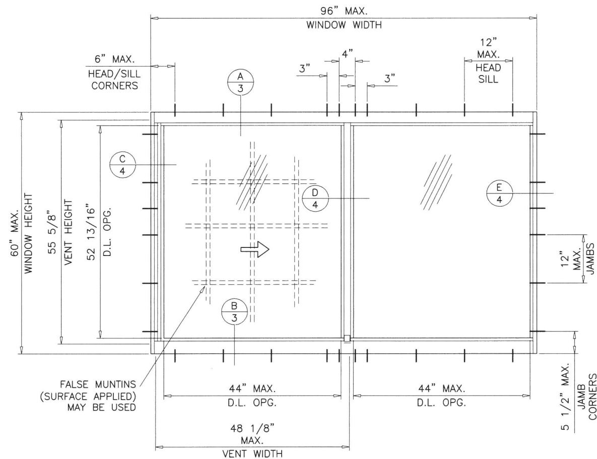
TYPICAL ELEVATION (TESTED UNIT)
